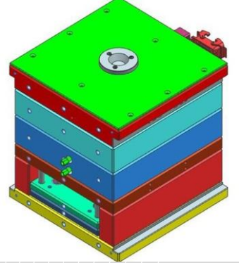
2 Plate Mould
