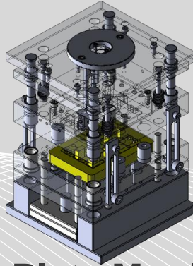
3 Plate Mould
